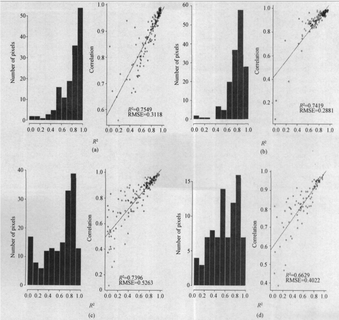
Fig. 3 Histograms of prediction R^2 , and the R^2 of correlations of LAI in 2007 with the mean LAI in 2001—2006 and the prediction R^2 of some land cover types (a) Croplands; (b) Mixed forest; (c) Evergreen forest; (d) Savannas
